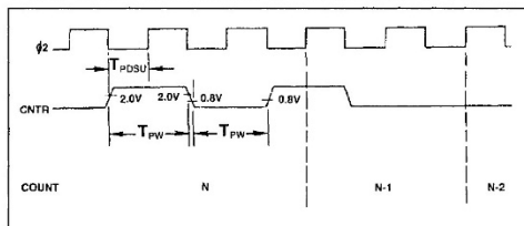
Figure 6-2. Event Counter Mode
