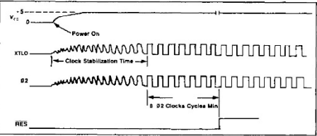
Figure 7-1. Power Turn-On Timing Detail
