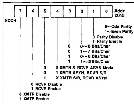
Figure 5-1. Serial Communication Control Register
