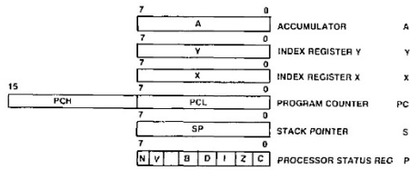
CPU Registers
