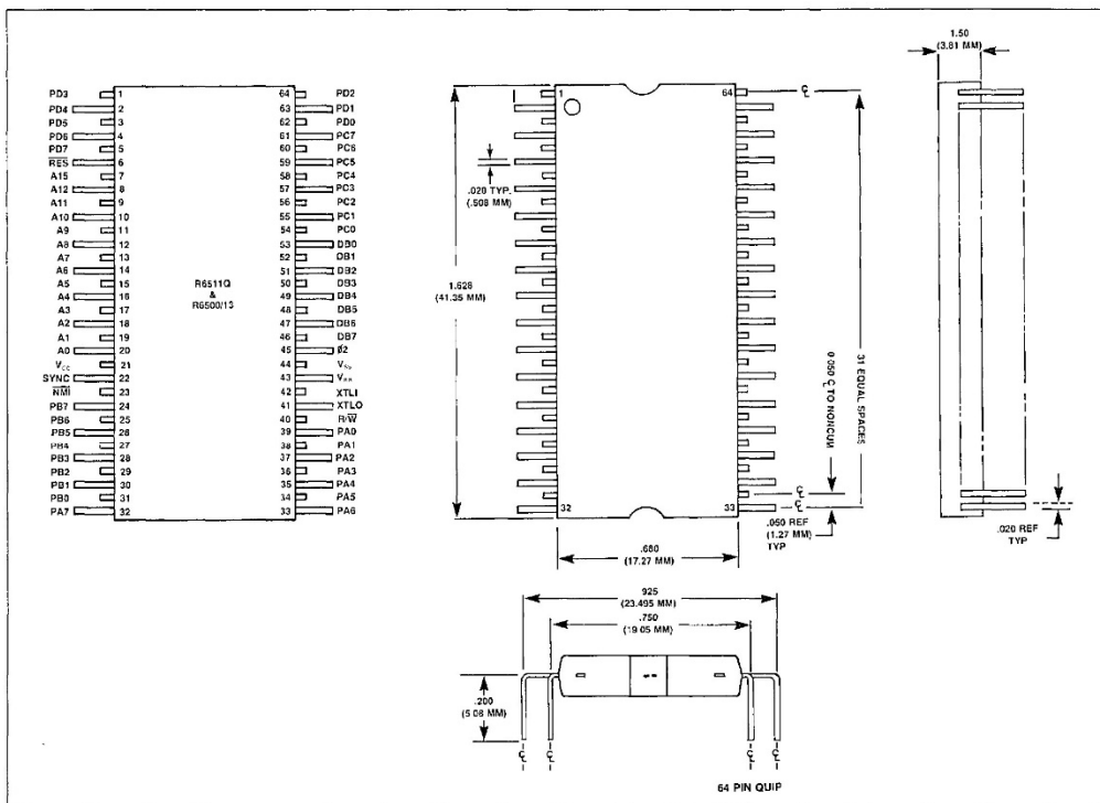
Figure 2-1. Mechanical Outline & Pin Out Configuration
