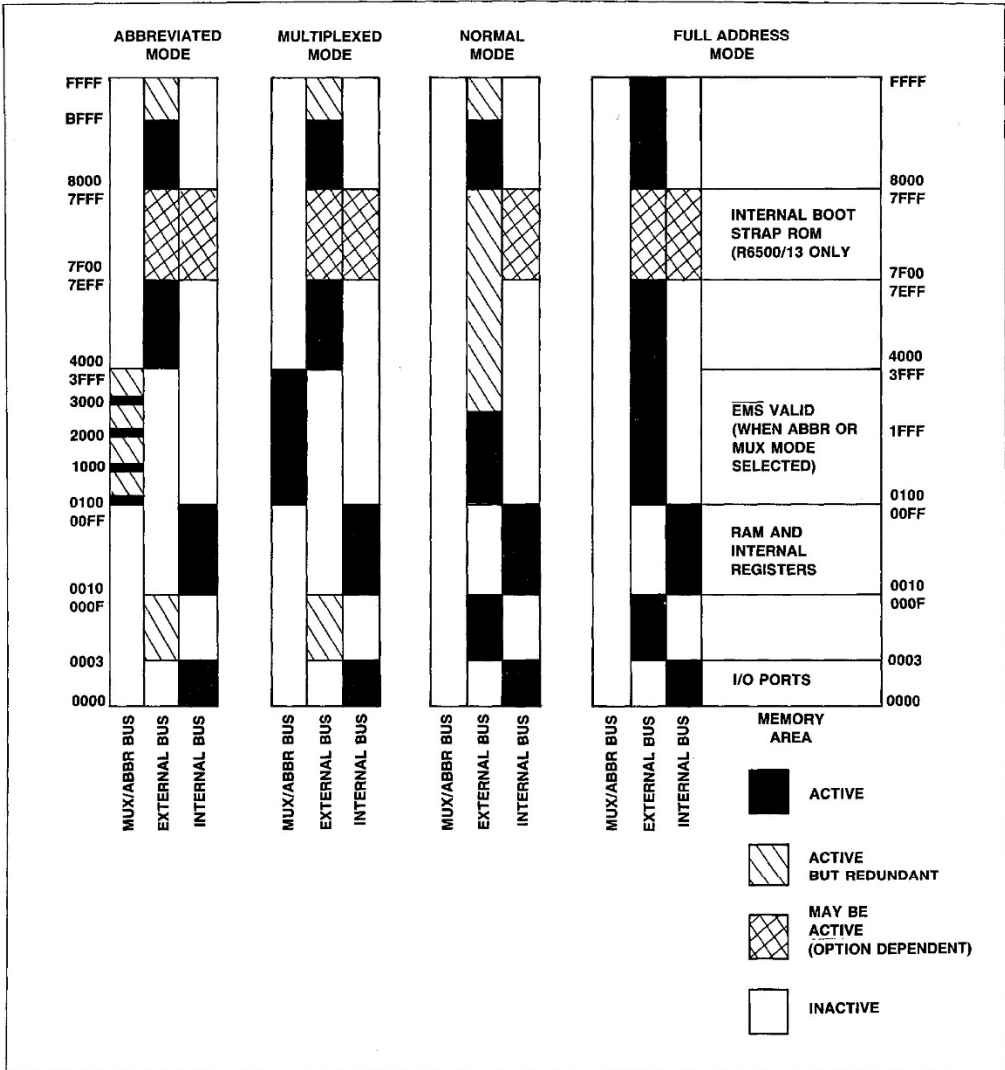
Figure 4-2. Memory Map
