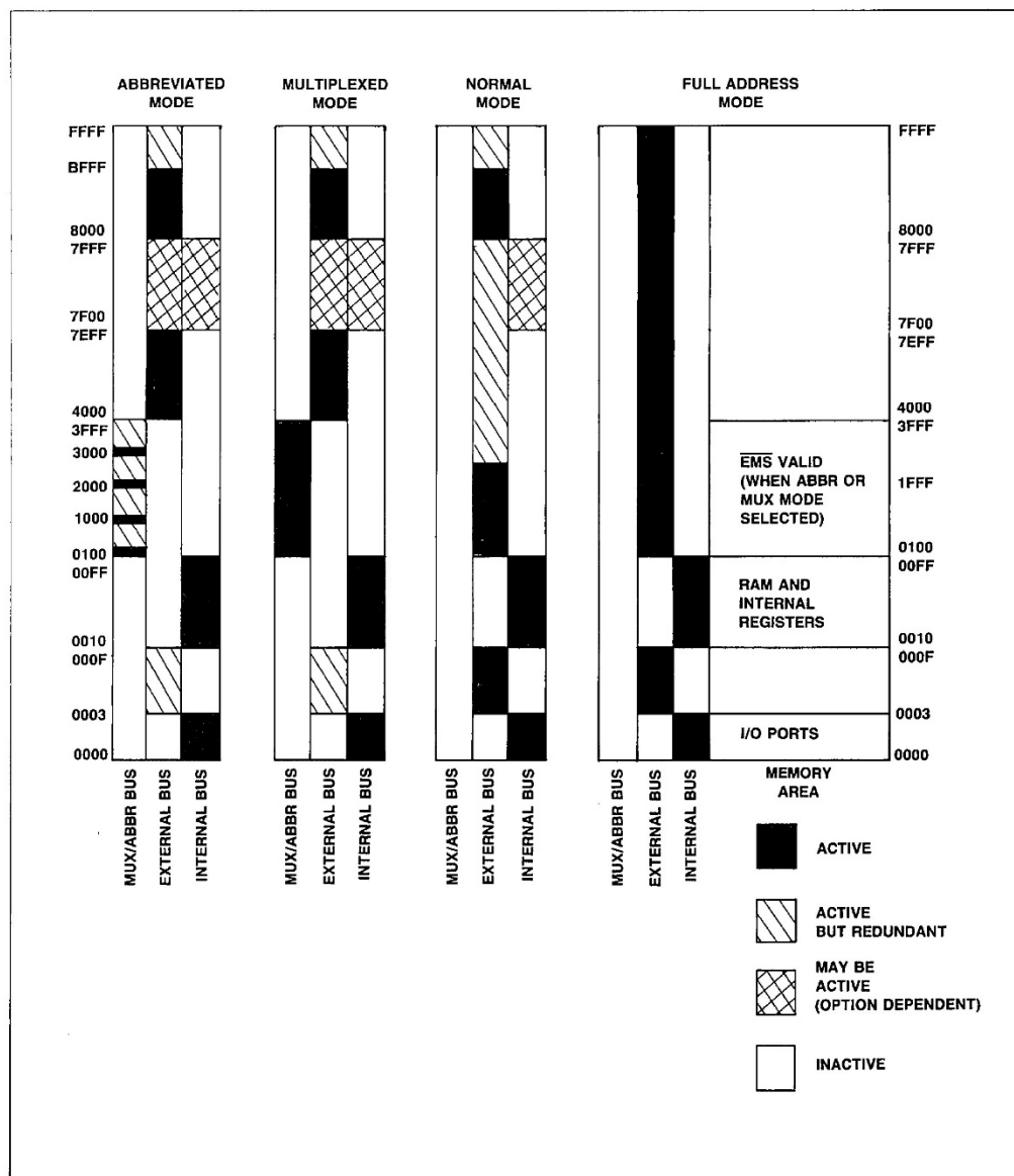
Figure 4-2. R6501 Memory Map
