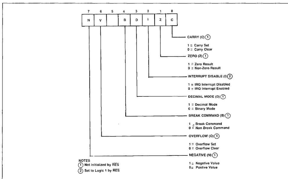
Figure 3-7. Processor Status Register
