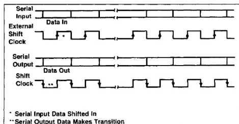
Figure 5-4. S/R Mode Timing
