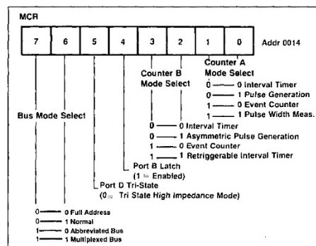
Figure 3-4. Mode Control Register
