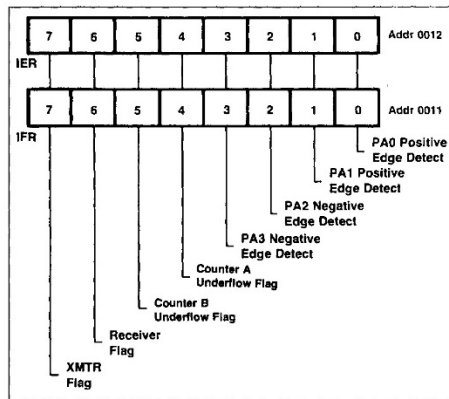
Figure 3-5. Interrupt Enable and Flag Registers
