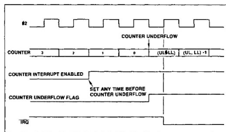
Figure 6-1. Interval Timer Timing Diagram
