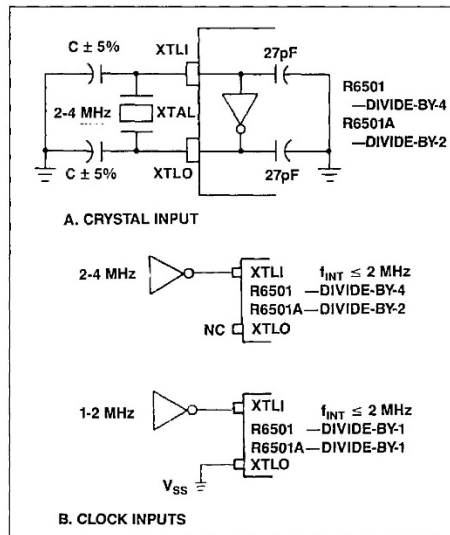
Figure 3-3. Clock Oscillator Input Options
