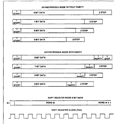
Figure 5-2. SIO Data Modes
