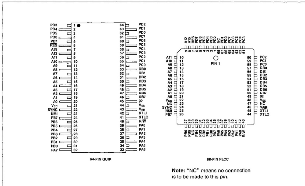
Figure 2-2. R6501 Pin Assignments
