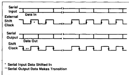
Figure 5-4. S/R Mode Timing
