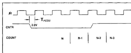
Figure 6-3. Pulse Width Measurement
