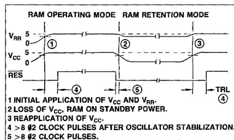
Figure 3-2. Data Retention Timing
