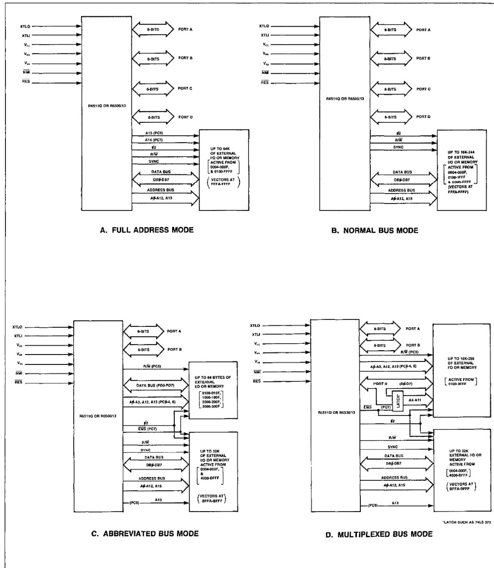
Figure 4-1. Bus Mode Configurations
