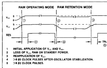
Figure 3-2. Data Retention Timing
