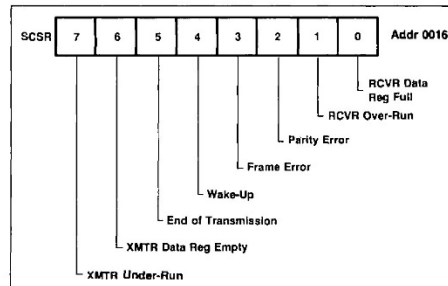
Figure 5-5. SCSR Bit Allocations
