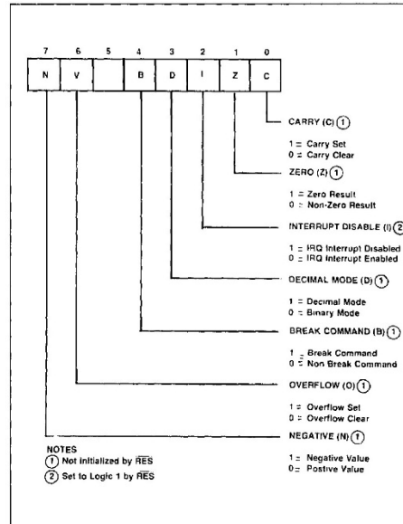
Figure 3-6. Processor Status Register
