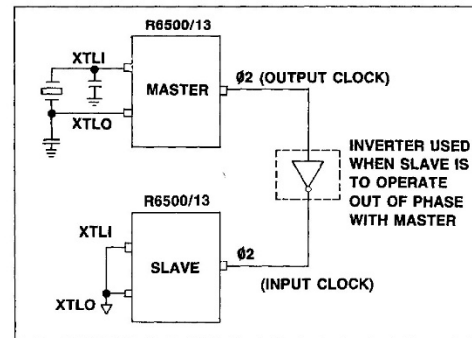
Figure 3-4. Master/Slave Connections
