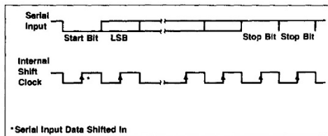
Figure 5-3. ASYN Receive Data Timing
