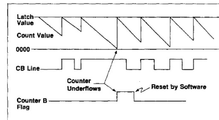
Figure 6-4. Counter B Retriggerable Interval Timer Mode
