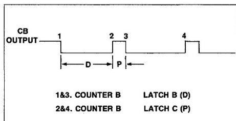
Figure 6-5. Counter B Pulse Generation
