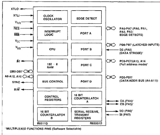
Figure 2-2. Interface Diagram
