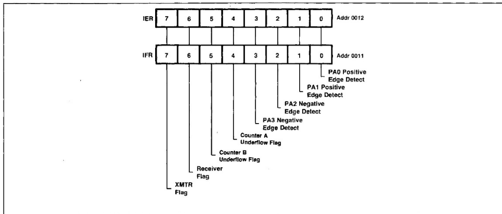
Figure 3-6. Interrupt Enable and Flag Registers
