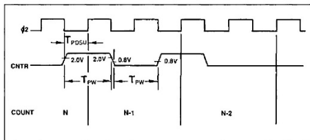
Figure 6-2. Event Counter Mode
