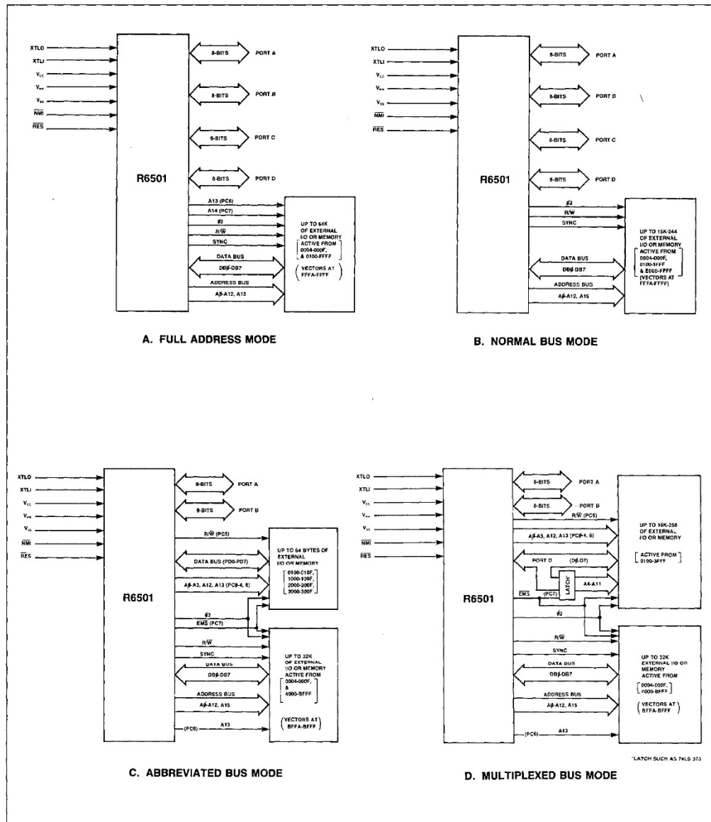
Figure 4-1. R6501 Bus Mode Configurations
