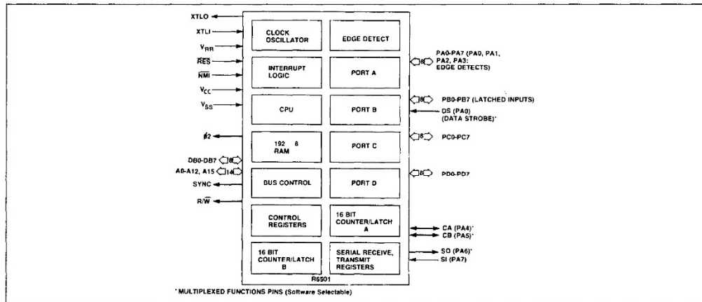
Figure 2-1. R6501 Interface Diagram
