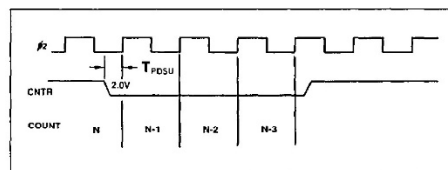
6-3. Pulse Width Measurement
