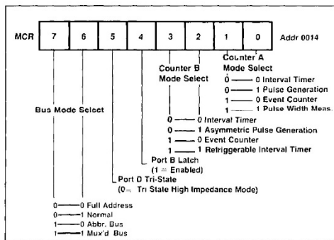
Figure 3-5. Mode Control Register
