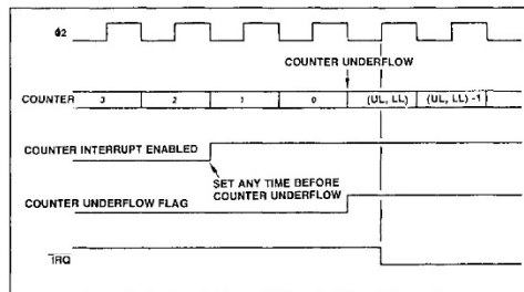
Figure 6-1. Interval Timer Timing Diagram
