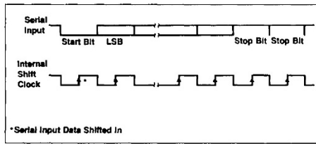
Figure 5-3. ASYN Receive Data Timing
