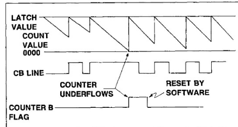
Figure 6-4. Counter B. Retriggerable Interval Timer Mode
