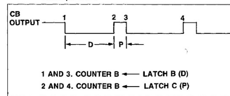
Figure 6-5. Counter B Pulse Generation
