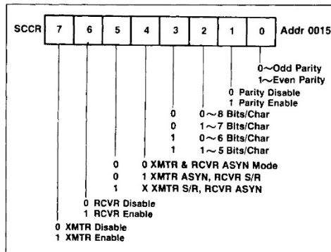
Figure 5-1. Serial Communication Control Register
