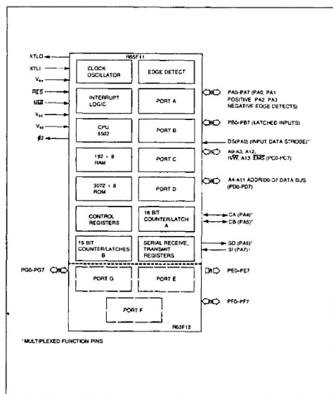
Figure 2-1. R65F11 and R65F12 Interface Diagram
