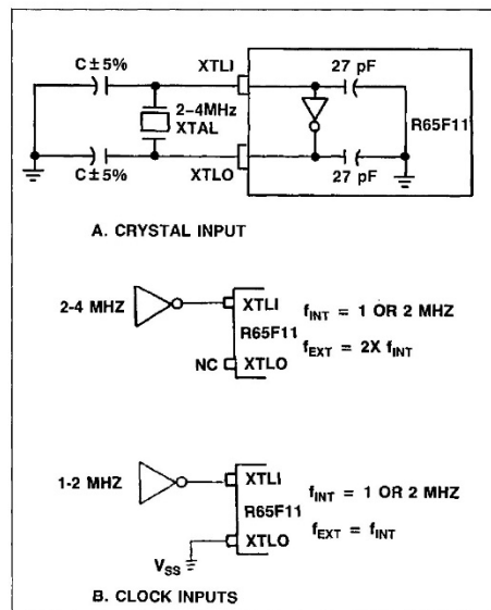
Figure 3-3. Clock Oscillator Input Options
