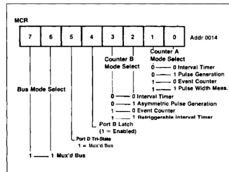
Figure 3-5. Mode Control Register
