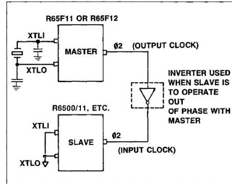
Figure 3-4. Master/Slave Connections
