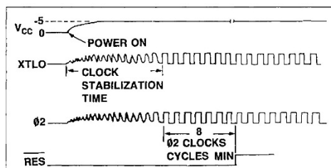
Figure 7-1. Power Turn-On Timing Detail
