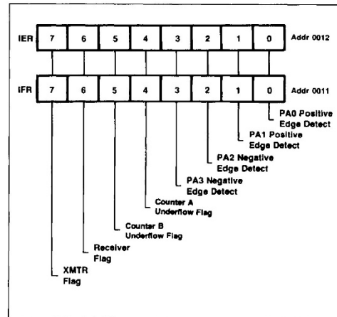
Figure 3-6. Interrupt Enable and Flag Registers
