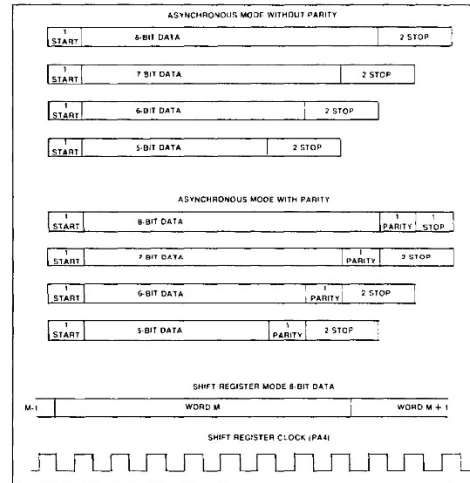
Figure 5-2. Bit Allocations
