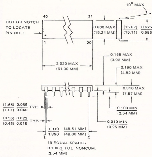
Packaging Diagram
