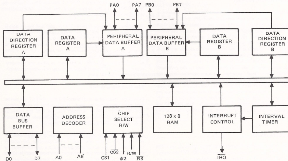
R6532 Block Diagram
