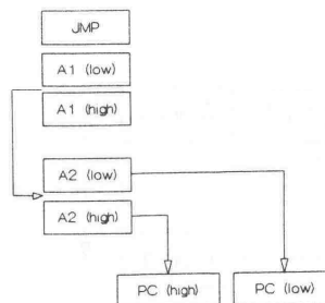
Fig. 5: JMP [A1]; Jump indirect
