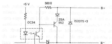
Transmission circuit
