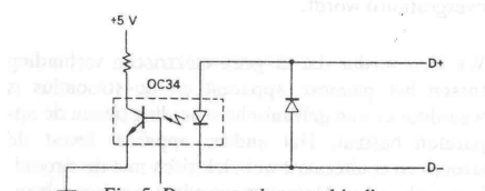
Fig. 5: De current loop verbinding
