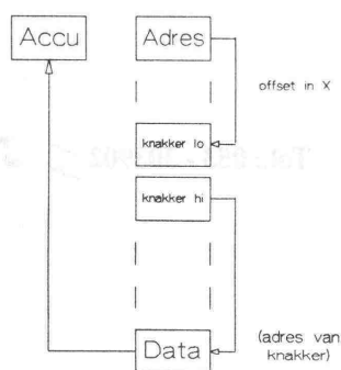
Fig. 6: LDA [ADRES,X]
