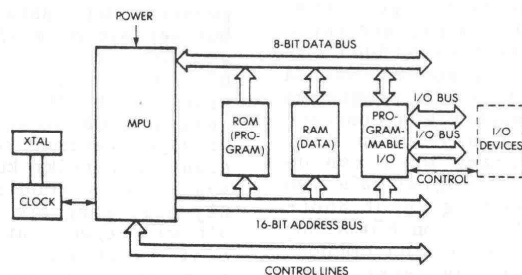
Fig. 3 : Architecture of a Standard Microprocessor System
