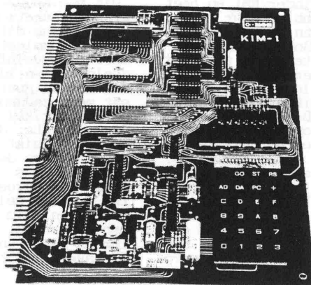
Fig. 1 : Photo of KIM-1
