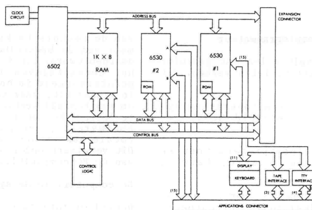
Fig. 2 : KIM-1 Internal Organization
