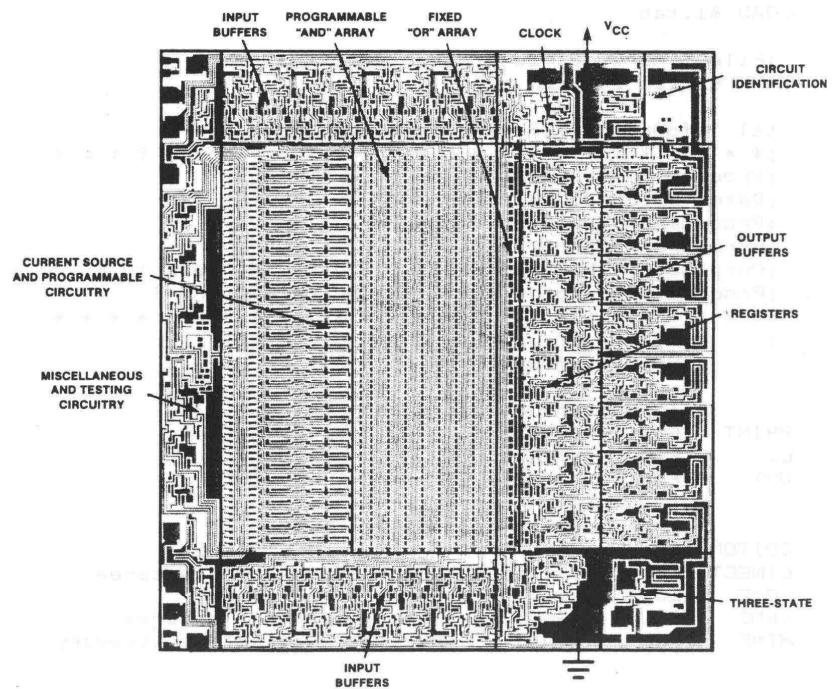
PAL 16R6 Metalization
