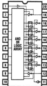
PAL16R6
