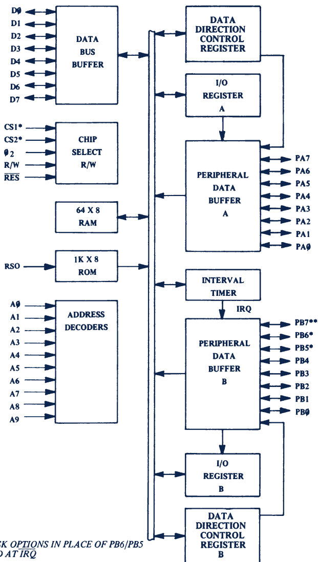
MCS6530 Internal Architecture FIGURE 1.33
