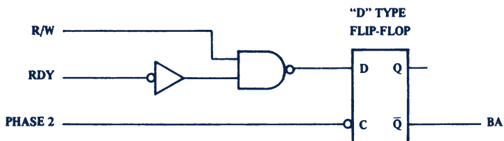
Logic Used to Generate Bus Available Signal for DMA Applications
