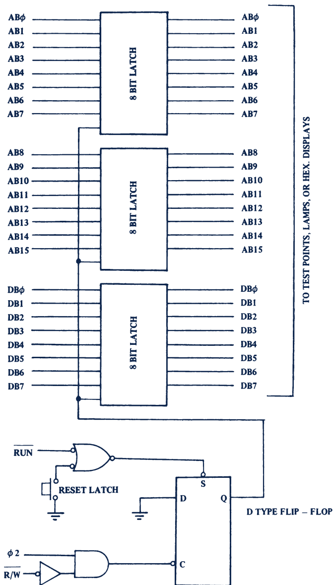
Microprocessor Single Cycle Data Trap
