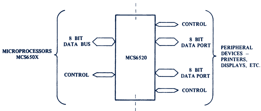
Basic MCS6520 Interface Diagram
