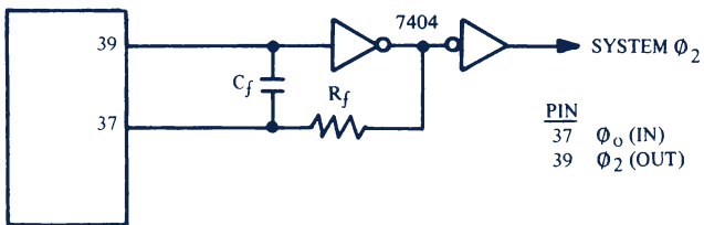
MCS6502 Time Base Generator - RC Network FIGURE 1.17
