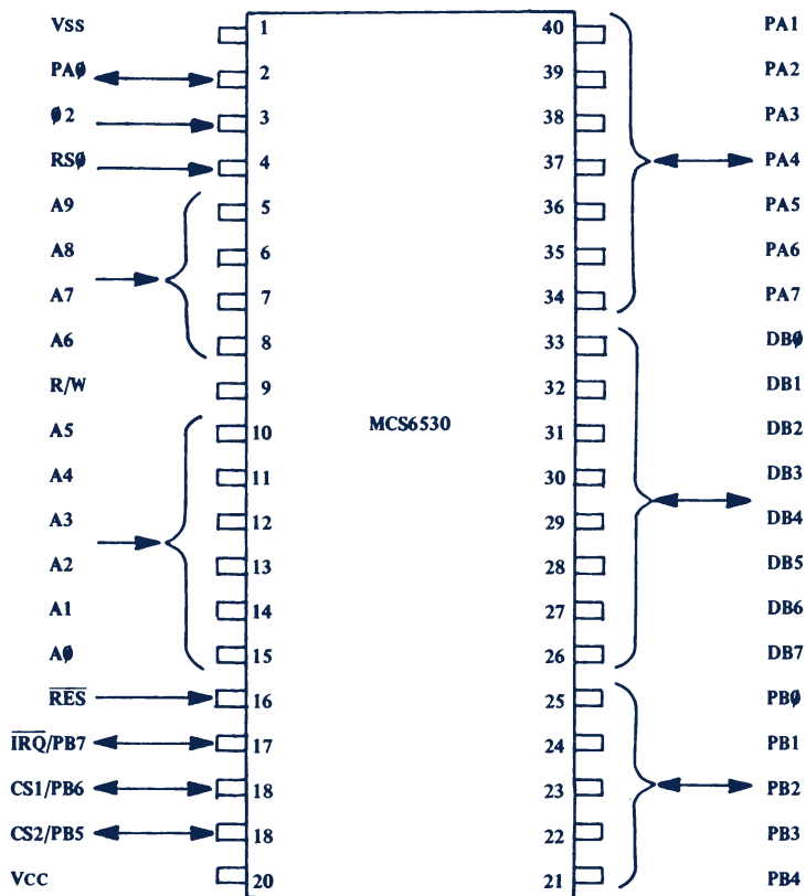
MCS6530 Pinout Designation
