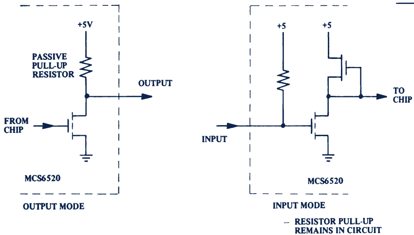
Peripheral I/O Port A Buffer FIGURE 1.28A
