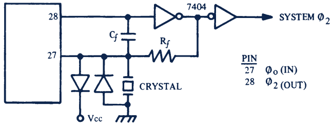
MCS6503,4,5 Parallel Mode Crystal Controlled Oscillator
