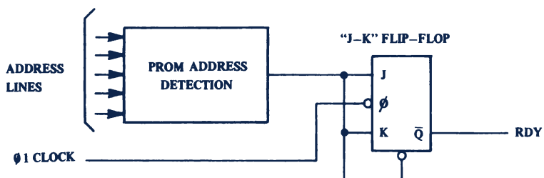
Interfacing Scheme for Slow PROM's
