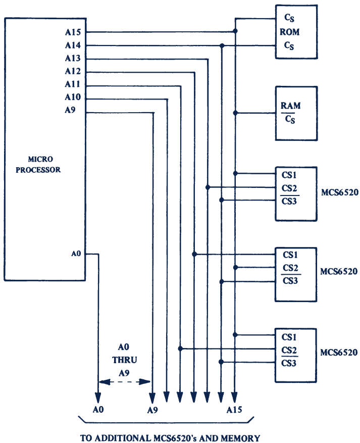
Typical Address Assignments FIGURE 2.10
