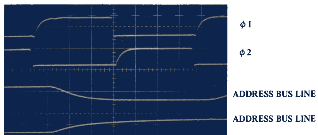
FIGURE 3.7b — Excess Address Line Loading
