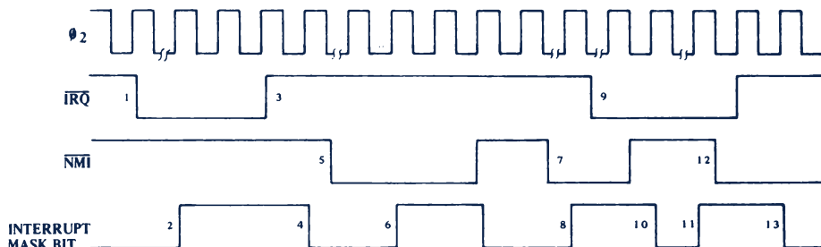
Examples of Interrupt Recognition by MCS650X
