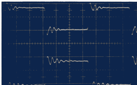
FIGURE 3.6a – Improper Clocks (Note undershoot and overlap)
