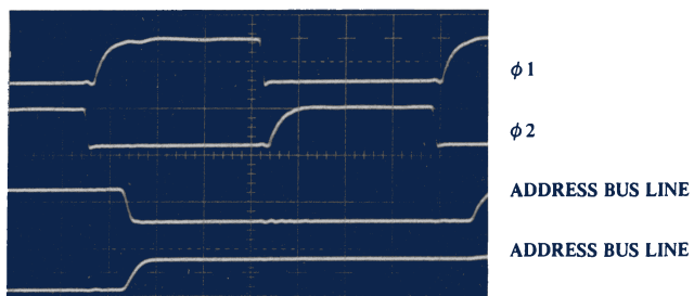
FIGURE 3.7a — Proper Address Lines
