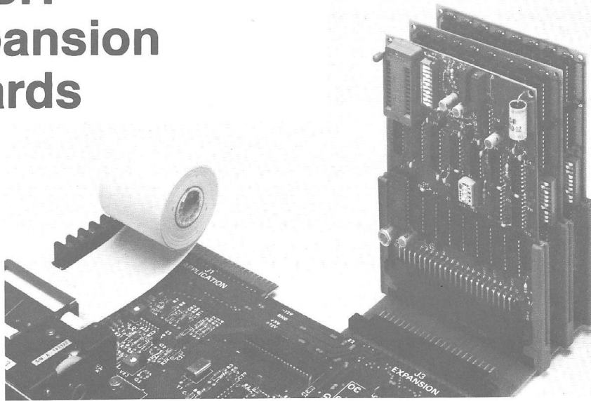
CUBIT Expansion Board Attached to AIM-65 Computer
