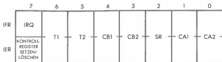
Abb. 9.10: Interrupt-Register
