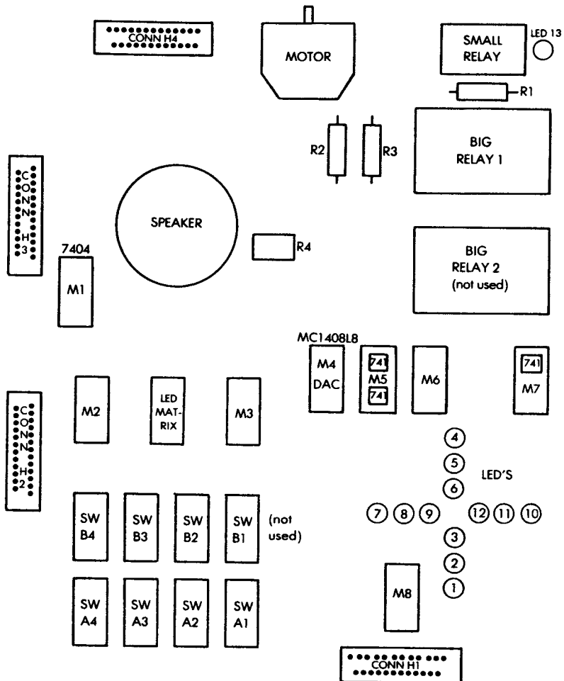
Fig. 5-4: Board Layout
