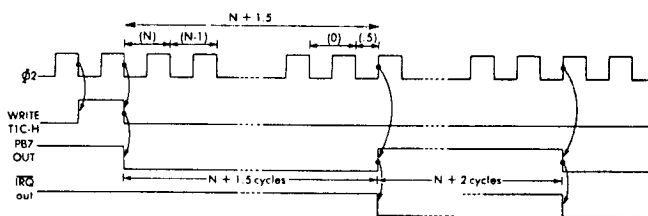
Fig. 4-26: Timing Diagram for Tone Generation
