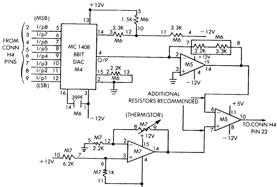
Fig. 5-47: ADC Interface
