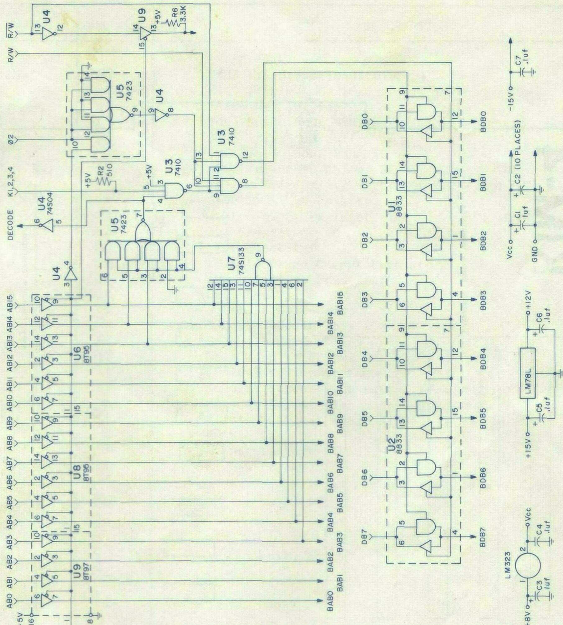
SCHEMATIC KIM-4
